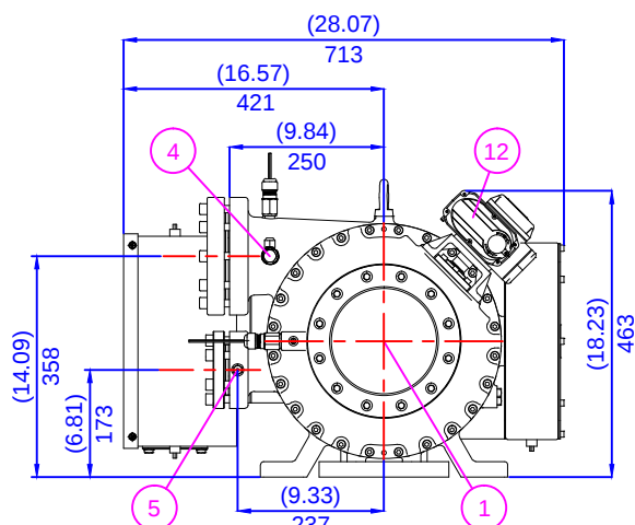
Left View
